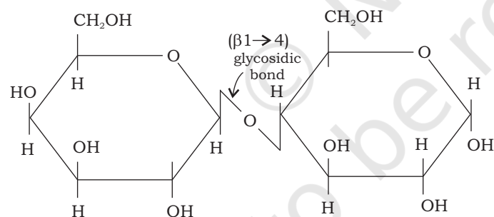
Fig. 3.7: Structure of lactose
